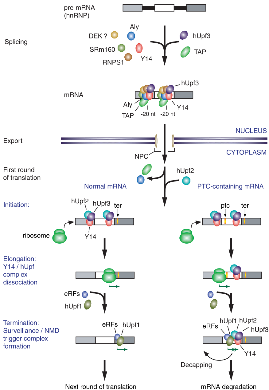
Fig. 5. A model depicting our view of the role of the exon-exon junction complex in providing a functional link among pre-mRNA splicing, nuclear export, and NMD of mRNA. The exon-exon junction complex comprises proteins that bind mRNAs that are produced by splicing in the nucleus. Several of the components of the complex remain associated with newly exported mRNAs (in the same position, 20 nt 5' to exon-exon junctions) in the cytoplasm. The pre-mRNAs are also with hnRNP proteins, which are omitted here for simplicity. See text for details. Abbreviations: PTC, premature termination codon/nonsense codon; NPC, nuclear pore complex; RF, translation release factor.
