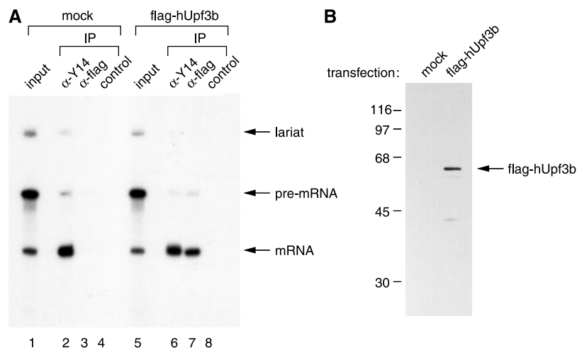
Fig. 3. hUpf3b is associated preferentially with spliced mRNA in vitro . (A) Immunoprecipitations were carried out after in vitro splicing of ^{32} P-labeled Ad2 pre-mRNA. For inclusion of Flag-hUpf3b in the reaction, HeLa nuclear extract was added with total cell extract from 293T cells that had been transfected with control plasmid (Flag-pcDNA3, lanes 1 to 4) or Flag-hUpf3b (lanes 5 to 8). Flag mAb M2, Y14 mAb 4C4, and control antibody (SP2/0) were used for immunoprecipitations. (B) Western blotting of the extracts from the cells transfected with control plasmid (mock) or Flag-hUpf3b (Flag-hUpf3b). The Flag-hUpf3b protein was detected using polyclonal rabbit antibody to Flag.
