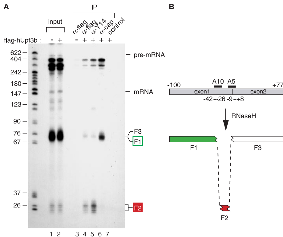
Fig. 4. hUpf3b is located immediately upstream of exon-exon junctions. (A) ^{32} P-labeled Ad2 pre-mRNA was incubated under in vitro splicing conditions as in Fig. 3 and subjected to RNase H digestion followed by immunoprecipitations and RNA analysis. Lanes 1 and 2 display the fragmentation pattern of RNAs after splicing and RNase H digestion. Lanes 3 to 7 show the fragments that were immunoprecipitated using the indicated antibodies. 293T cells had been transfected with control plasmid (Flag-pcDNA3, lanes 1 and 3) or Flag-hUpf3b (lanes 2 and 4 to 7). Flag mAb, Y14 mAb 4C4, cap mAb H20, and control nonimmune antibody (SP2/0) were used for immunoprecipitations. (B) Positions of the oligonucleotides and the RNA fragments from the spliced Ad2 mRNA are depicted. The red box indicates the fragment bound to hUpf3b and Y14 (F2). The green box indicates the 5'-most fragment (F1).
