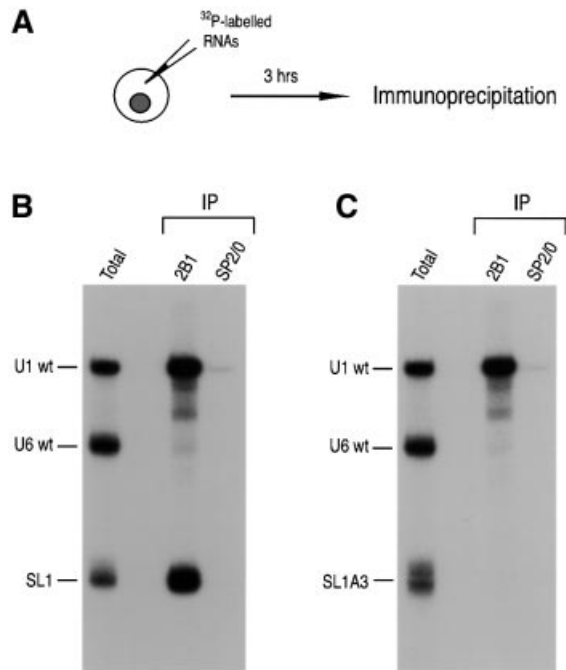
Fig. 3. Sequence-specific interaction of the SMN complex with SL1 of U1 snRNA. (A) Experimental strategy used in this experiment. A mixture of 32 P-labeled RNAs was injected into the cytoplasm of oocytes. Following a 3 h incubation, the oocytes were homogenized, and immunoprecipitated with 2B1 or SP2/0 antibodies. Immunoprecipitated RNAs were analyzed as described in Figure 2B. (B) SL1 is sufficient for U1 snRNA interaction with the SMN complex. A mixture of 32 P-labeled U1, U6 snRNAs and SL1 was microinjected and analyzed as described in (A). (C) The SMN complex binding to the SL1 of U1 snRNA is sequence specific. A mixture of 32 P-labeled U1, U6 snRNAs and SL1A3 was microinjected and analyzed as described in (A).
