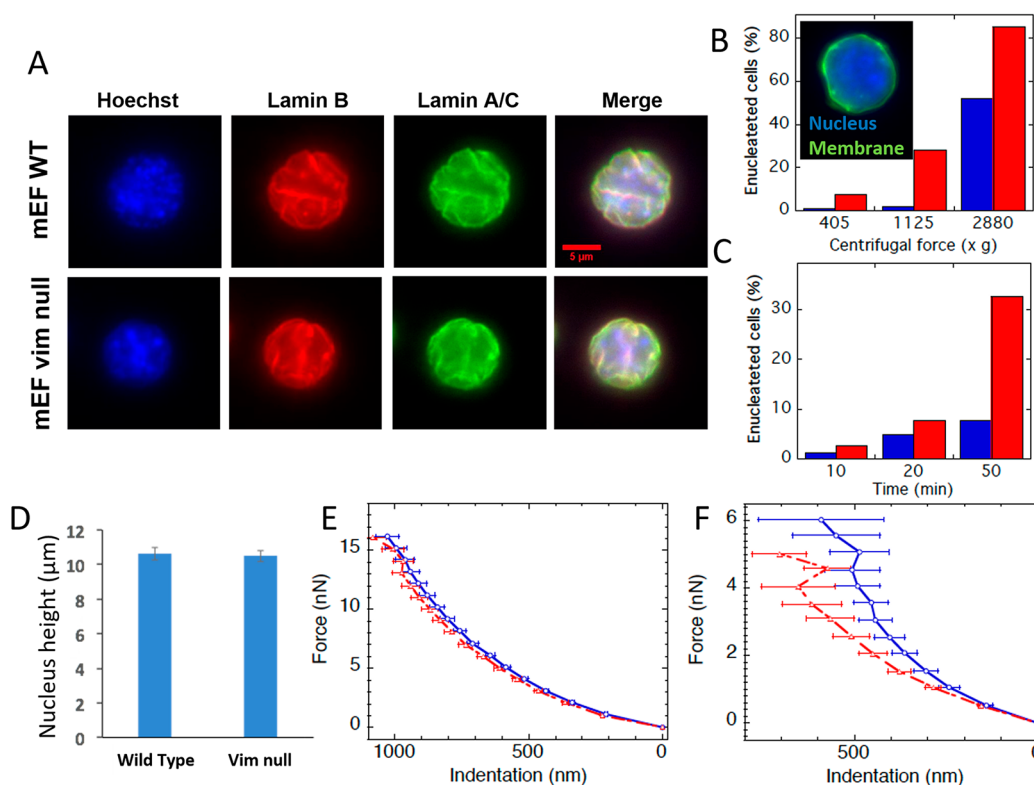
Figure 3. Mechanical response of a single nucleus isolated from the wild type and vimentin null mEFs. (A) Fluorescence staining of the nucleus isolated from wild type and vimentin null mEFs (scale bar 5 \mu\text{m} ). (B) Percent of the enucleated cells as a function of centrifugal force. (C) Percent of enucleated cells as a function of centrifugation time. (D) Nucleus height of the wild type mEF and vim null mEFs as determined using AFM. (E) Force versus indentation curve for the nucleus isolated from wild type mEFs (blue) and vim null mEF (red). (F) Force versus indentation curve for the nucleus-free cytoplasts from wild type mEFs (blue) and vim null mEFs (red).
