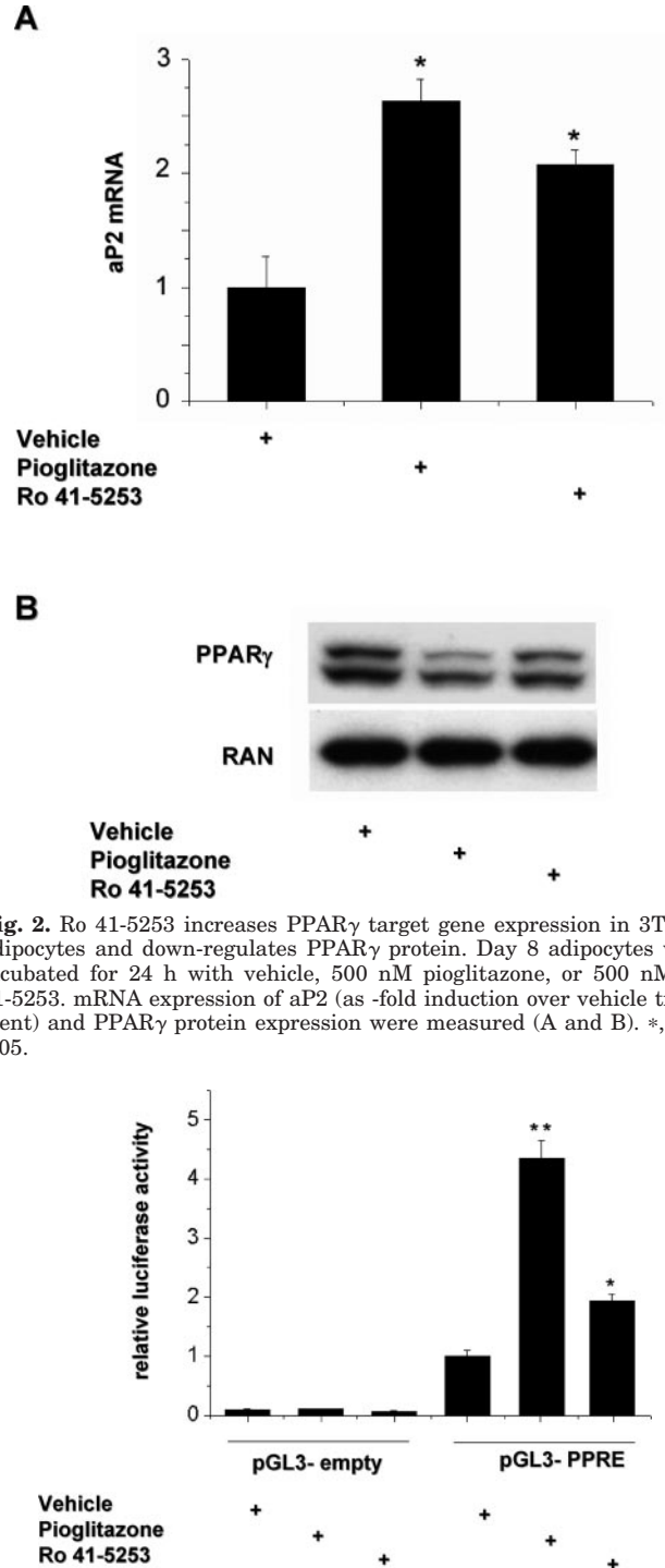
Fig. 3. Ro 41-5253 increases endogenous PPAR activity in adipocytes. 3T3-L1 adipocytes were electroporated with either empty vector (pGL3) or a PPAR- response element containing reporter (pGL3-3xAOx-PPRE) and incubated for 24h with vehicle and 500 nM pioglitazone or 500 nM Ro 41-5253 and assayed for luciferase activity. Data represent the -fold induction of luciferase activity over vehicle treatment of the PPRE-containing plasmid. *, p < 0.05 ; **, p < 0.01 .
