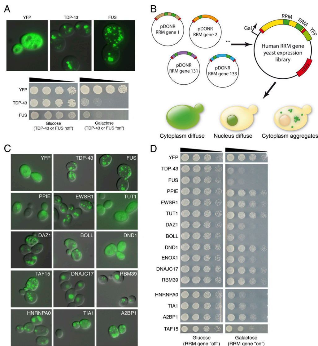
Fig. 1. A yeast functional screen identifies human RRM proteins with properties similar to FUS and TDP-43. (A) When expressed in yeast, TDP-43 and FUS form multiple cytoplasmic aggregates (Upper) and are toxic (Lower). (B) We designed a yeast functional screen to identify additional human RRM proteins that aggregate and are toxic in yeast. A library of 133 different human ORFs encoding the proteins was cloned into yeast expression vectors as galactose-inducible YFP fusions. We individually transformed each of these plasmids into yeast cells and assessed their effect on aggregation and toxicity by fluorescence microscopy and spotting assays, respectively. (C) Examples of various localization patterns in yeast cells of human RRM proteins. Some proteins were localized diffusely throughout the cytoplasm (TUT1 and DND1) and others were localized diffusely in the nucleus (DNAJC17). Some formed multiple foci in the nucleus (RBM39) and several others resembled FUS and TDP-43, which formed multiple cytoplasmic foci (EWSR1, TAF15, HNRNPA0, and DAZ1). (D) Spotting assays to assess the toxicity of human RRM proteins. Transformants were grown on synthetic media containing either glucose (control, RRM gene "off") or galactose (to induce expression of candidate ORFs, RRM gene "on"). Some proteins were very toxic when overexpressed (DAZ1, HNRNPA0, FUS, and TDP-43) whereas others were moderately toxic (EWSR1 and TAF15) and others were not toxic (PPIE and DNAJC17). See Table 1 and Dataset S1 for toxicity and aggregation scores.
