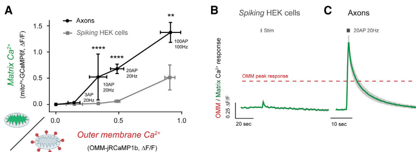
AP at 20 Hz in neurons and the equivalent \text{Ca}^{2+} increase in the OMM of HEK cells, measured by quantifying OMM \text{Ca}^{2+} signals (red) in both cell types (traces not shown for clarity, but average OMM peak response is denoted with a red dashed line). Experiments were performed in the presence of glucose. Error bars indicate SEM. **p < 0.01, ****p < 0.0001, Mann-Whitney U test.
