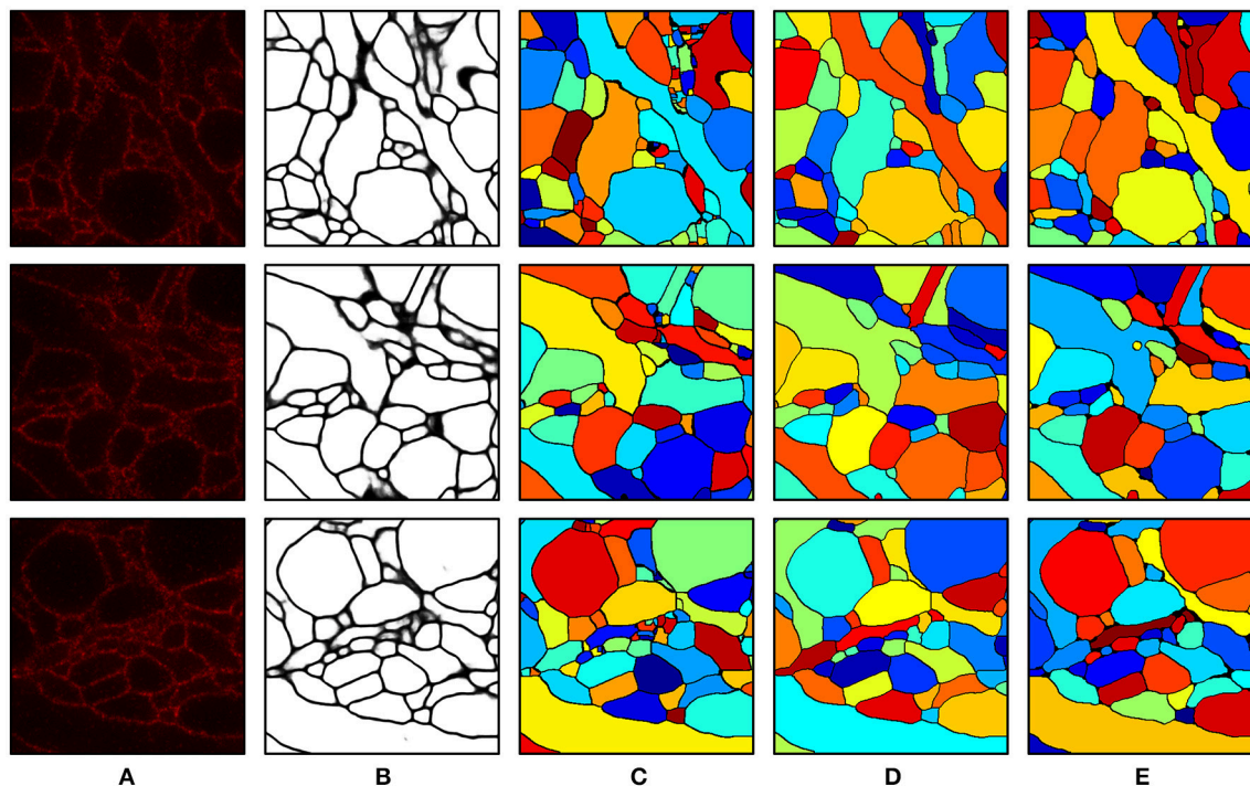
FIGURE 7 | Segmentation results. (A) Input image. (B) Boundary probability map. (C) Initial over-segmentation obtained by applying watershed transformation to the boundary probability map. (D) Final segmentation obtained by agglomerating (C) using GALA and barcodes. Barcodes with a density of 30 barcodes/ \mu\text{m}^3 were used for the agglomeration. (E) Ground truth. The field of view of each image is 2.4 \times 2.4 \mu\text{m} .
