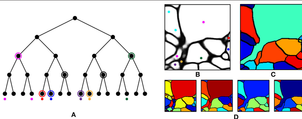
FIGURE 6 | Agglomeration algorithm using barcodes. (A) Illustration of our agglomeration algorithm using hierarchical segmentation tree and barcodes. Here, the hierarchical segmentation is obtained by applying GALA to the initial over-segmentation with different threshold values. Colored dots represent barcodes and their colors represent their identity. Highest levels of the nodes are found (circled) that do not contain different barcodes (as would result from a strategy of merging whenever barcodes do not mismatch). (B) Barcodes (represented as colored dots) overlaid on the boundary probability map. Each color represents a unique sequence of barcodes. (C) Final segmentation obtained by using the barcodes in (B) and the hierarchical segmentation tree in (D) . (D) Four levels of hierarchical segmentation from GALA.
