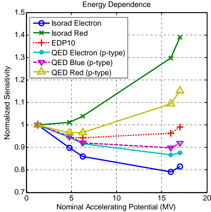
Figure 20. Energy dependence for different (old) diodes.
