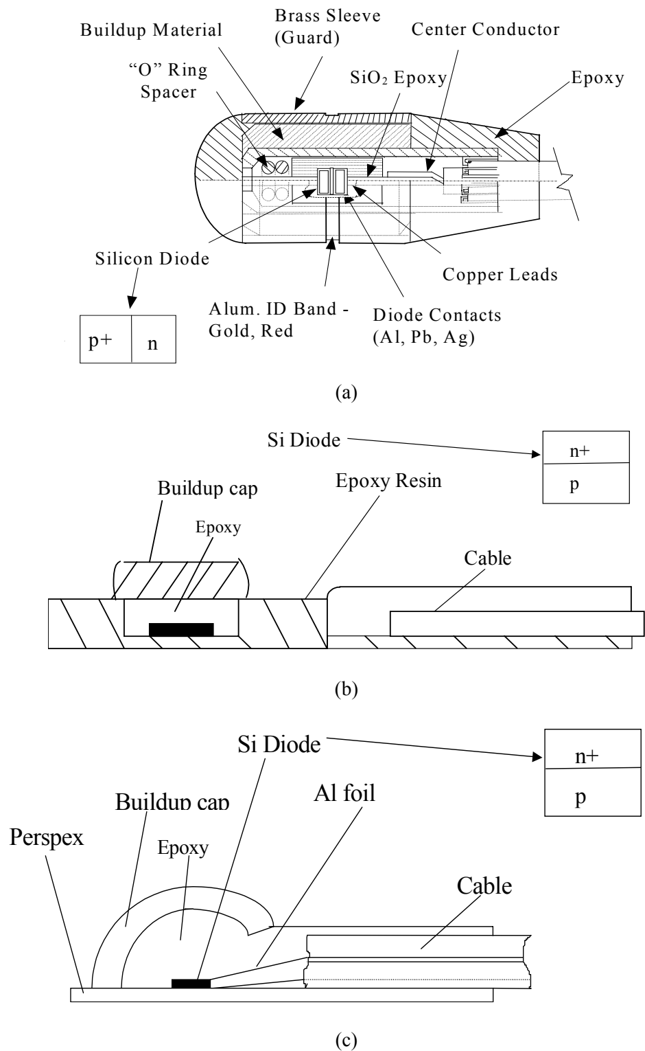
Figure 5. The schematics of the patient dosimetry diode detectors. (a) Isorad, (b) QED, (c) EDP.
