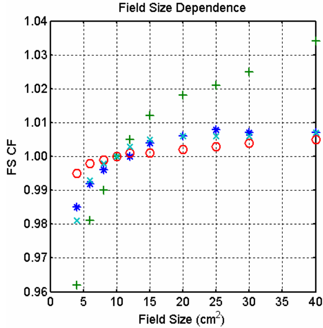
Figure 25. Field size dependence correction factors for different diodes.
