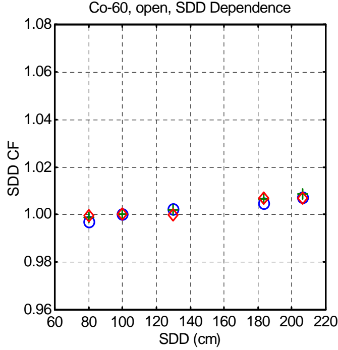
Figure 14. SDD dependence of different diodes under Co-60 radiation. o - Isorad Gold #2, + - Isorad Red (n-type), and ◇ - EDP30.
