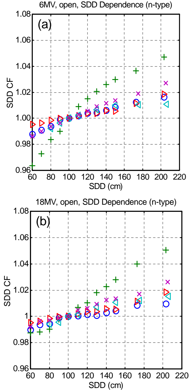
Figure 12. SDD correction factors for n-type diodes under pulsed beams. (a) 6 MV and (b) 18 MV. o - Isorad Gold #1, + - Isorad Red (n-type), Δ - Isorad-3 Gold, < - Veridose Green, and x - QED Red (n-type).
