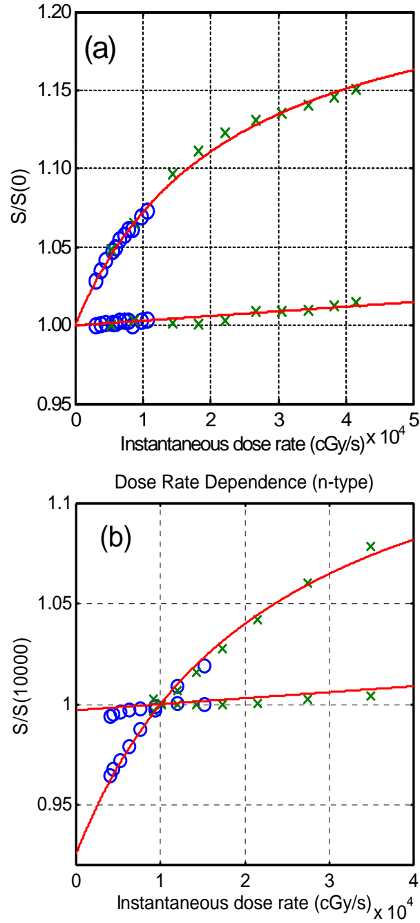
Figure 16. Dose rate dependence of an n-type and a p-type diode detectors. Measured by (a) adjusting the radiation pulse height directly at a fixed SDD and field size (SDD = 67.5 cm, 25 \times 25 cm 2 , d = 3.5 cm) and (b) SDD measurement under otherwise the same conditions. From top to bottom, the curves are for Isorad Gold #2 (n-type) and EDP30, p-type. The symbols are for different photon energies: o – 8 MV, x – 18 MV. Solid lines are fits using Eq. (53) (Fig. 16a) and Eq. (52) (Fig. 16b) with the same parameters in Table 6 (see text for details).
