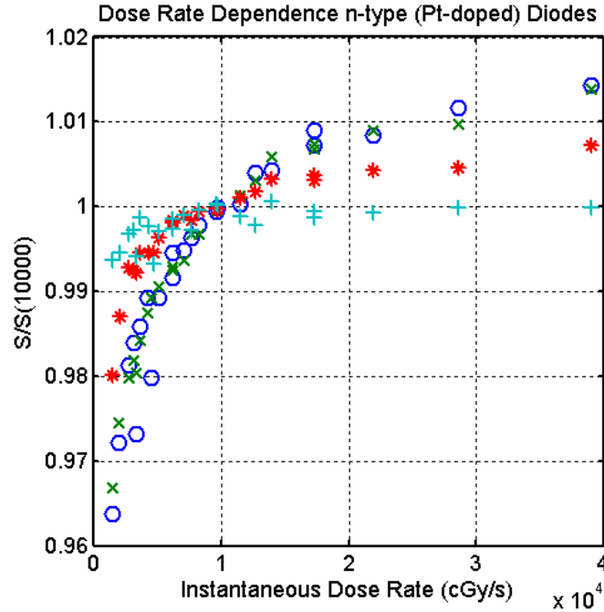
Figure 24. Dose rate dependence of pt-doped diode detectors (6 and 18 MV).
