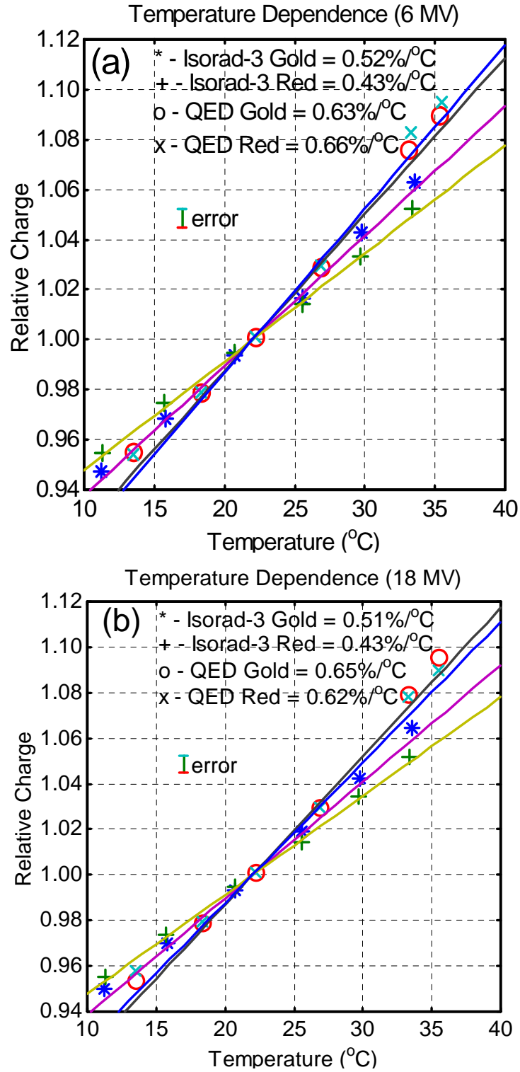
Figure 27. Temperature dependence for different diode detectors. (a) 6 MV (b) 18 MV, * - Isorad-3 Gold, + - Isorad-3 Red, O - QED Gold, and x - QED Red.
