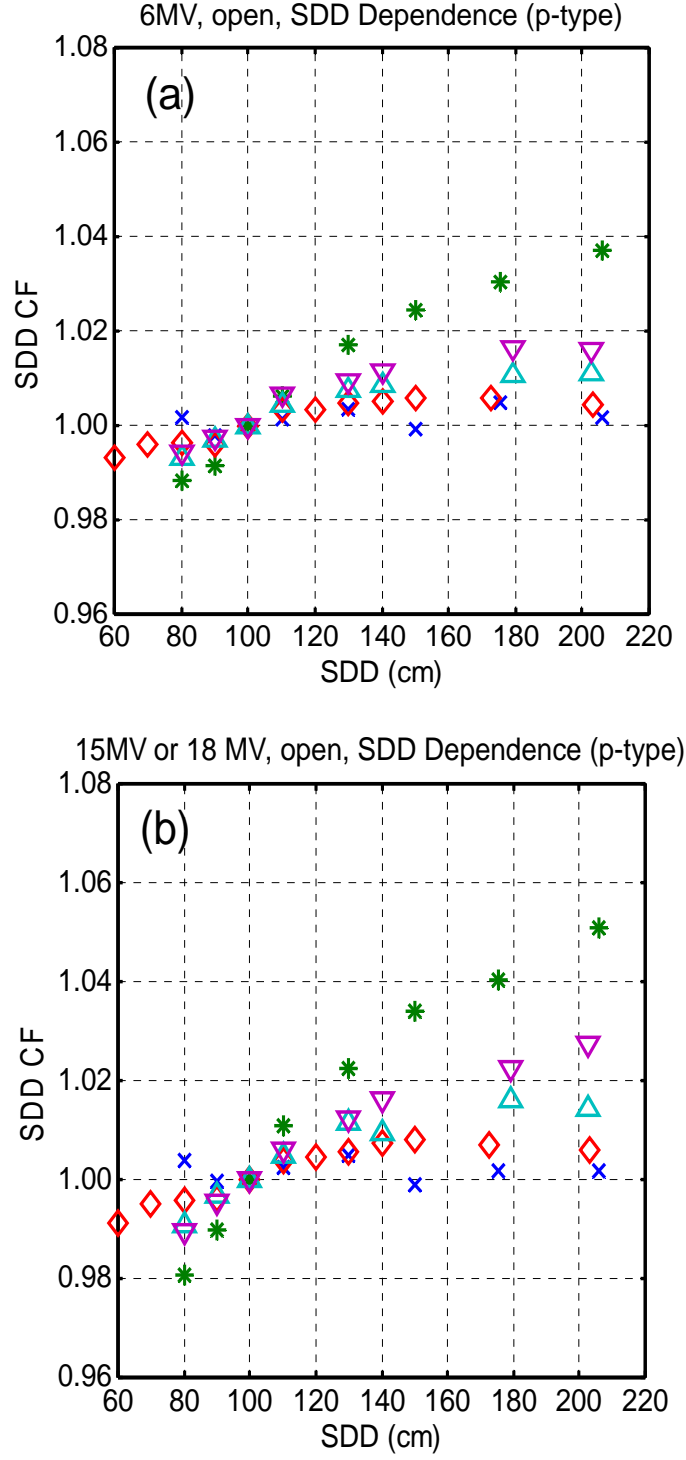
Figure 13. SDD correction factors for p-type diodes under pulsed beams. (a) 6 MV and (b) 15 or 18 MV. \diamond - EDP10 3G , \times - EDP20 3G , * - Isorad Red (p-type), \Delta - QED Red (p-type), and \nabla - QED Blue.
